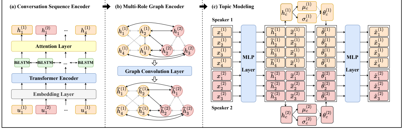
Figure 1: The model overview of ConvNTM: a) The conversation sequence encoder for modeling the multi-turn conversation contexts; b) The multi-role graph encoder for formulating the intra-speaker and inter-speaker dependencies; c) The topic modeling module to reconstruct utterance-level BoWs based on fusion of global and local topic information.
