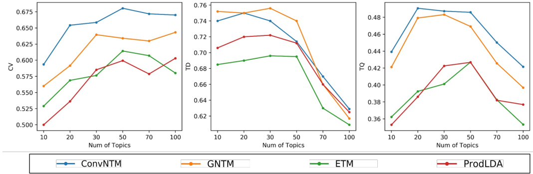
Figure 2: Comparison results of the varying number of topics on DailyDialog.
